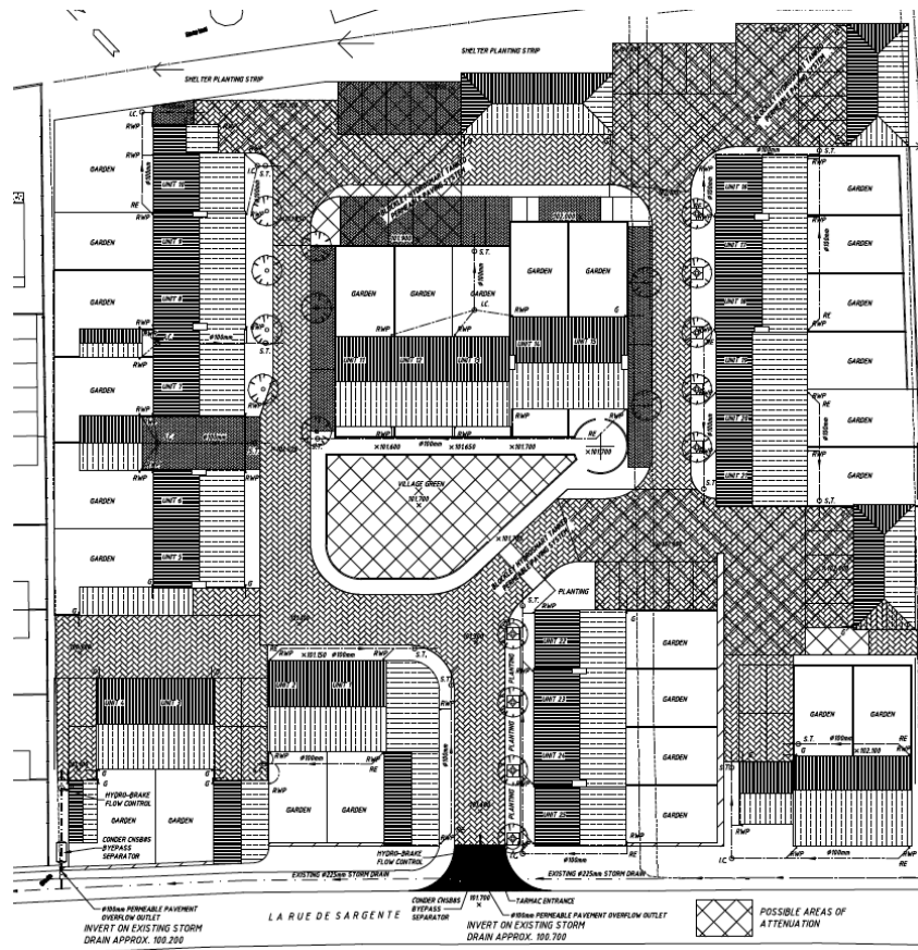
Figure 1. The roads and parking areas on this project were surfaced with permeable paving.
