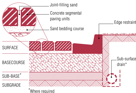
Figure 1 Concrete segmental pavement structure
